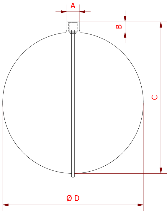
Misure d'ingombro - Overall dimensions (mm)
