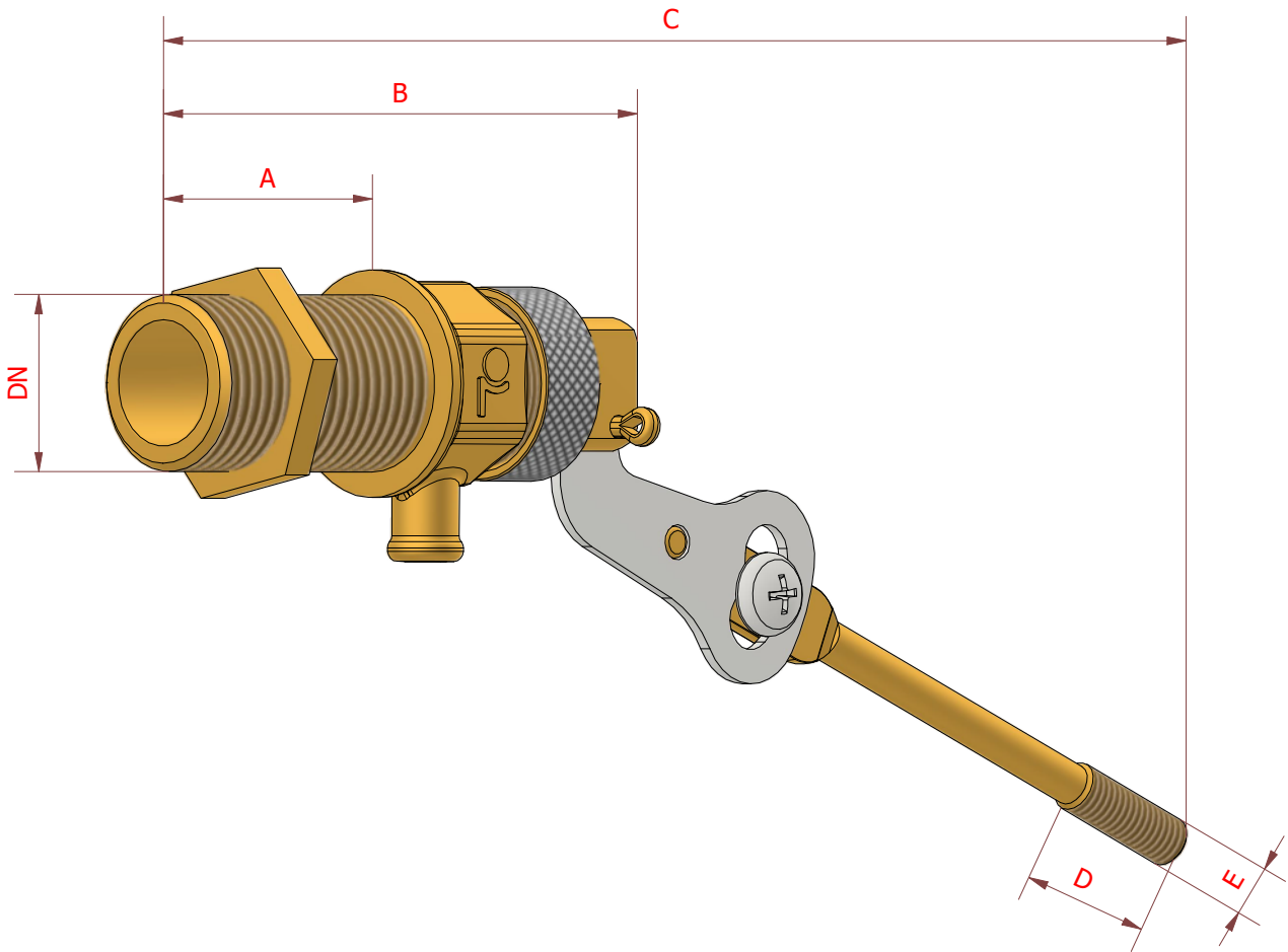
Misure d'ingombro - Overall dimensions (mm)
