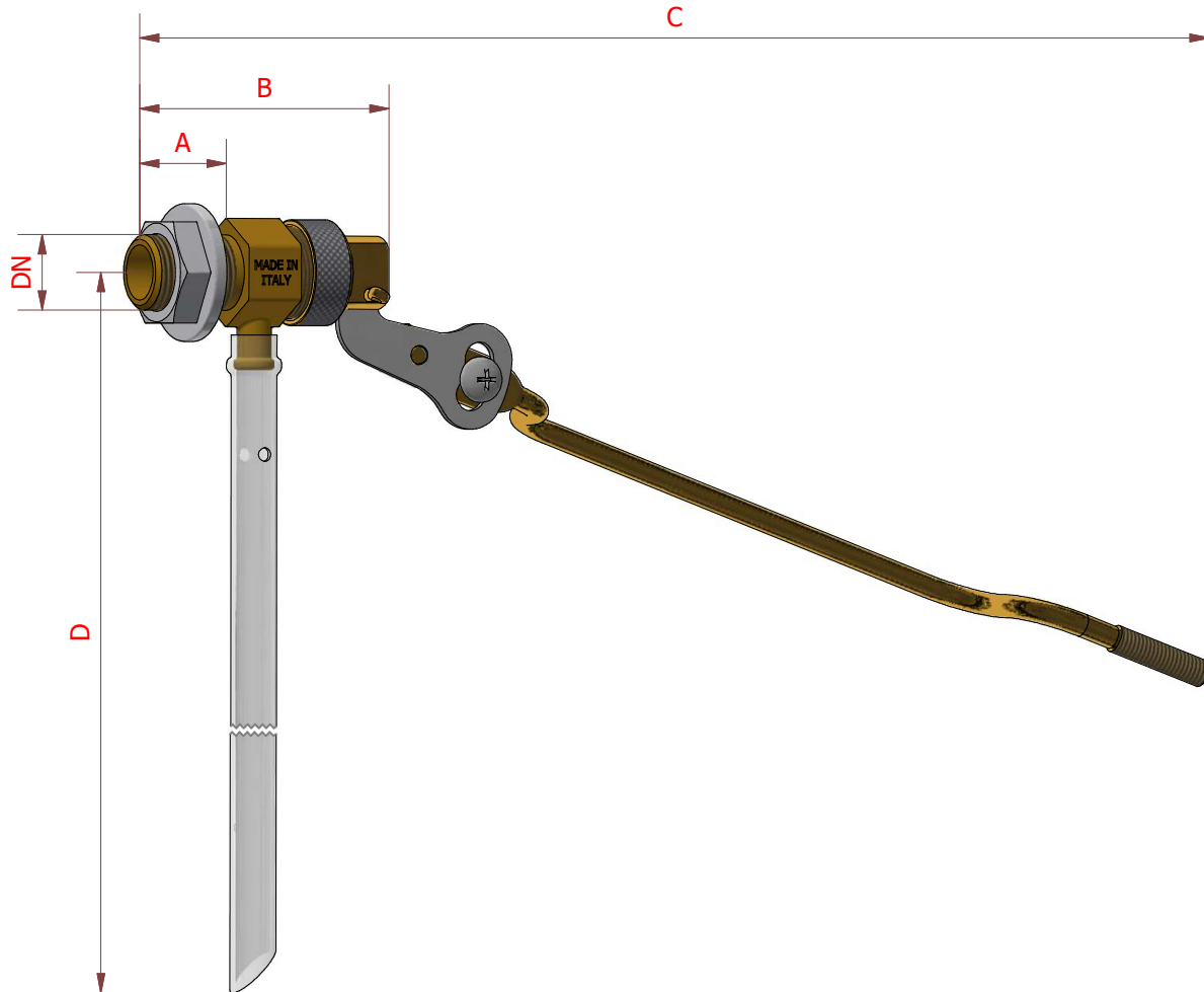
Misure d'ingombro - Overall dimensions (mm)
