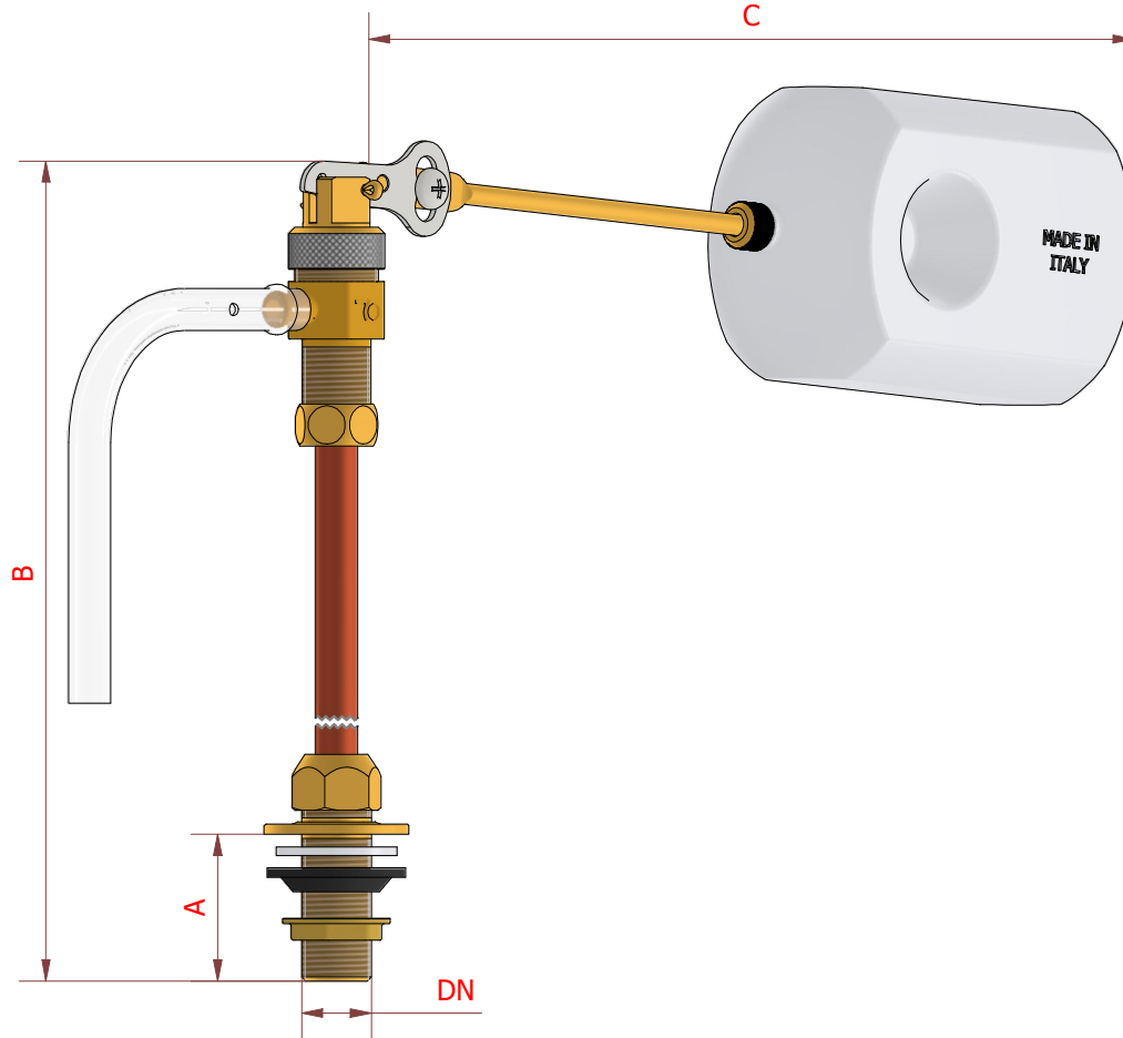
Misure d'ingombro - Overall dimensions (mm)
