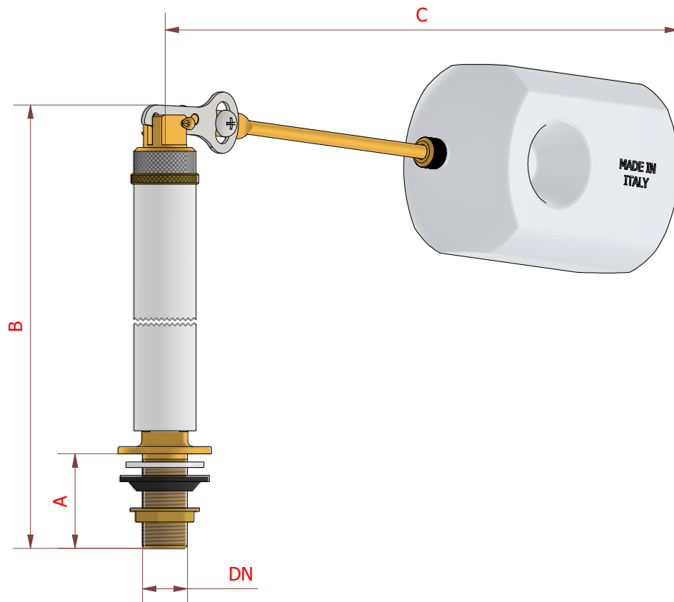
Misure d'ingombro - Overall dimensions (mm)
