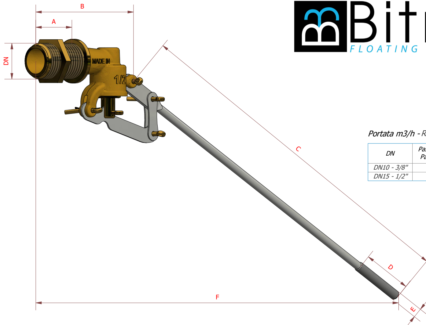
Misure d'ingombro - Overall dimensions (mm)
