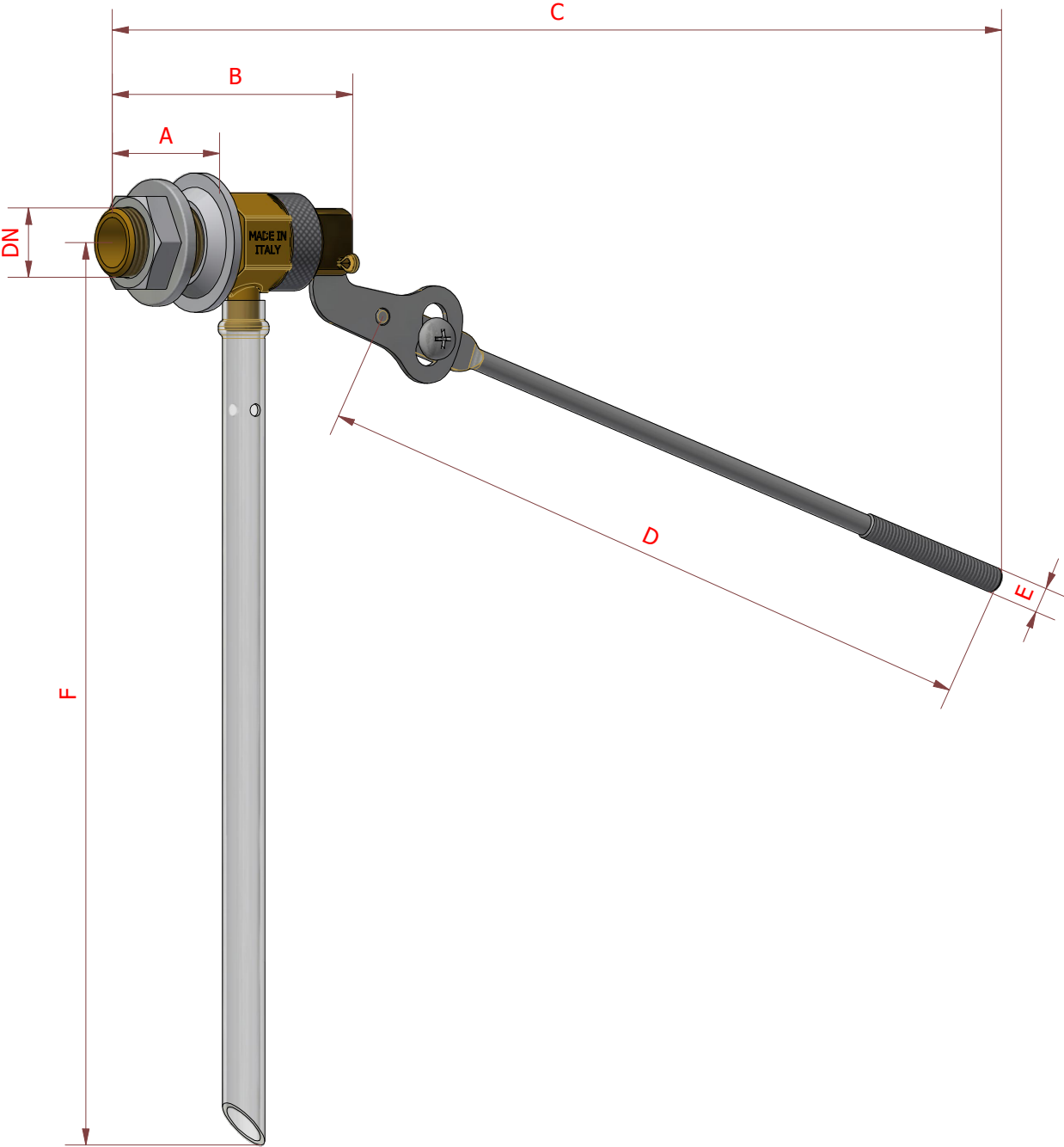
Misure d'ingombro - Overall dimensions (mm)
